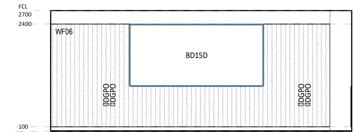
3 ELEVATION DETAIL 60-029 1 : 50
