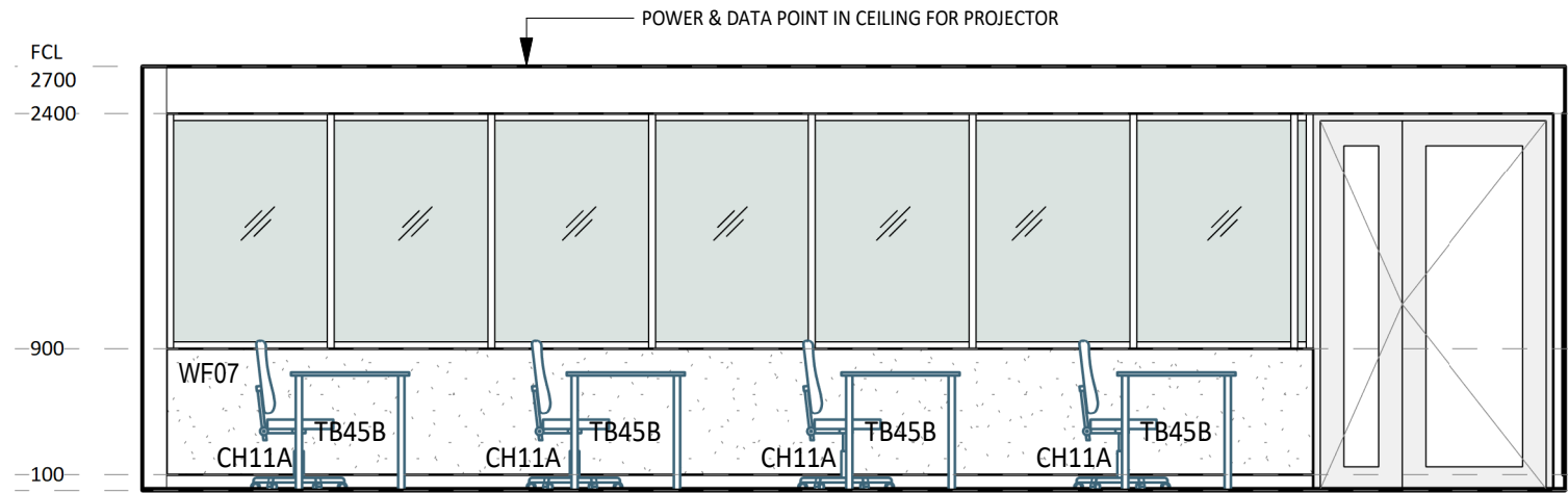
2 ELEVATION DETAIL 60-025 1 : 50
