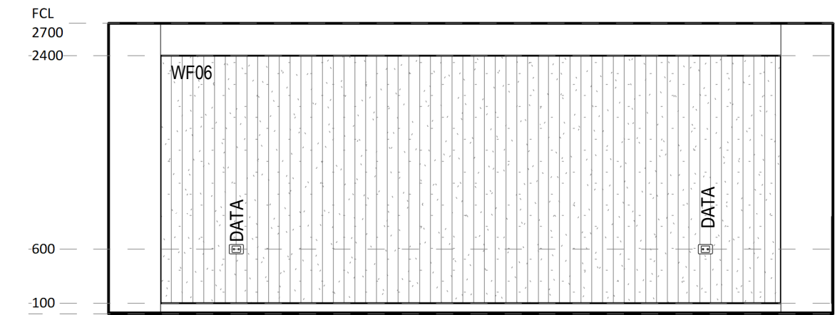
4 ELEVATION DETAIL 60-029 1 : 50
