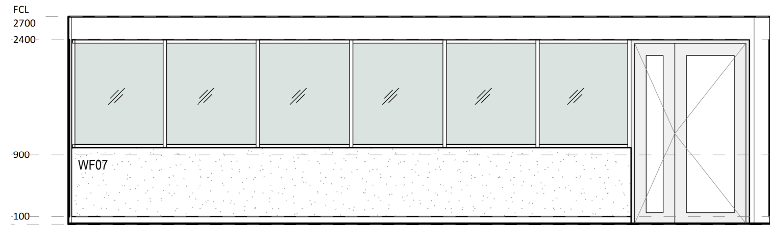
5 ELEVATION DETAIL 60-019 1 : 50
